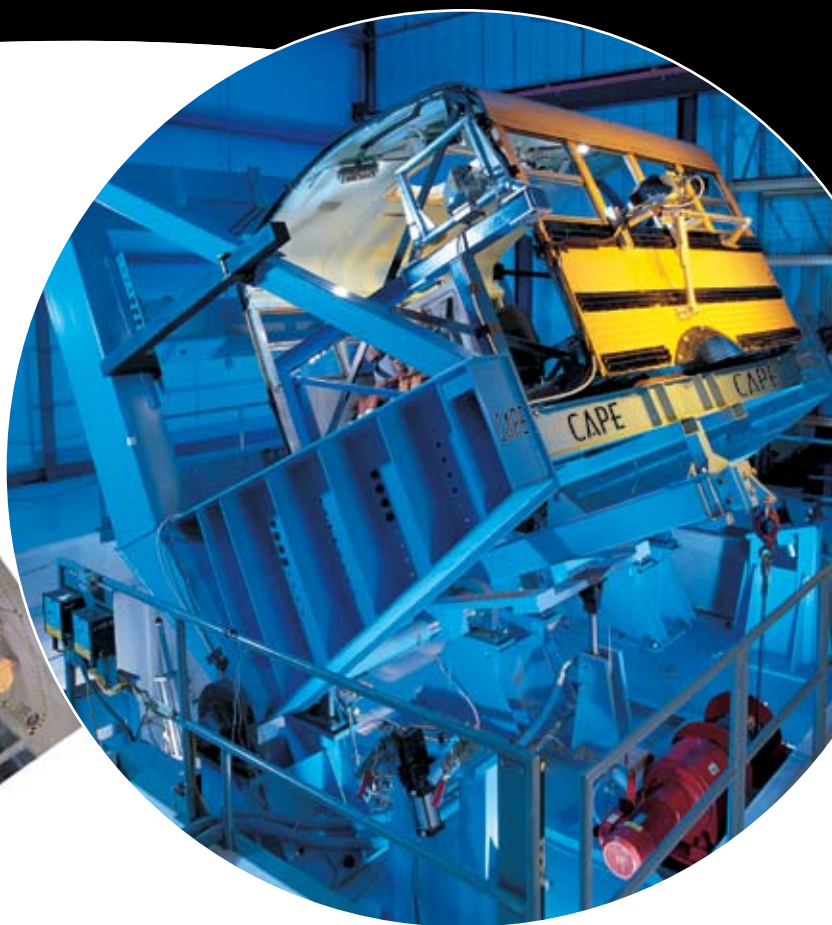
School bus body section on rollover machine
